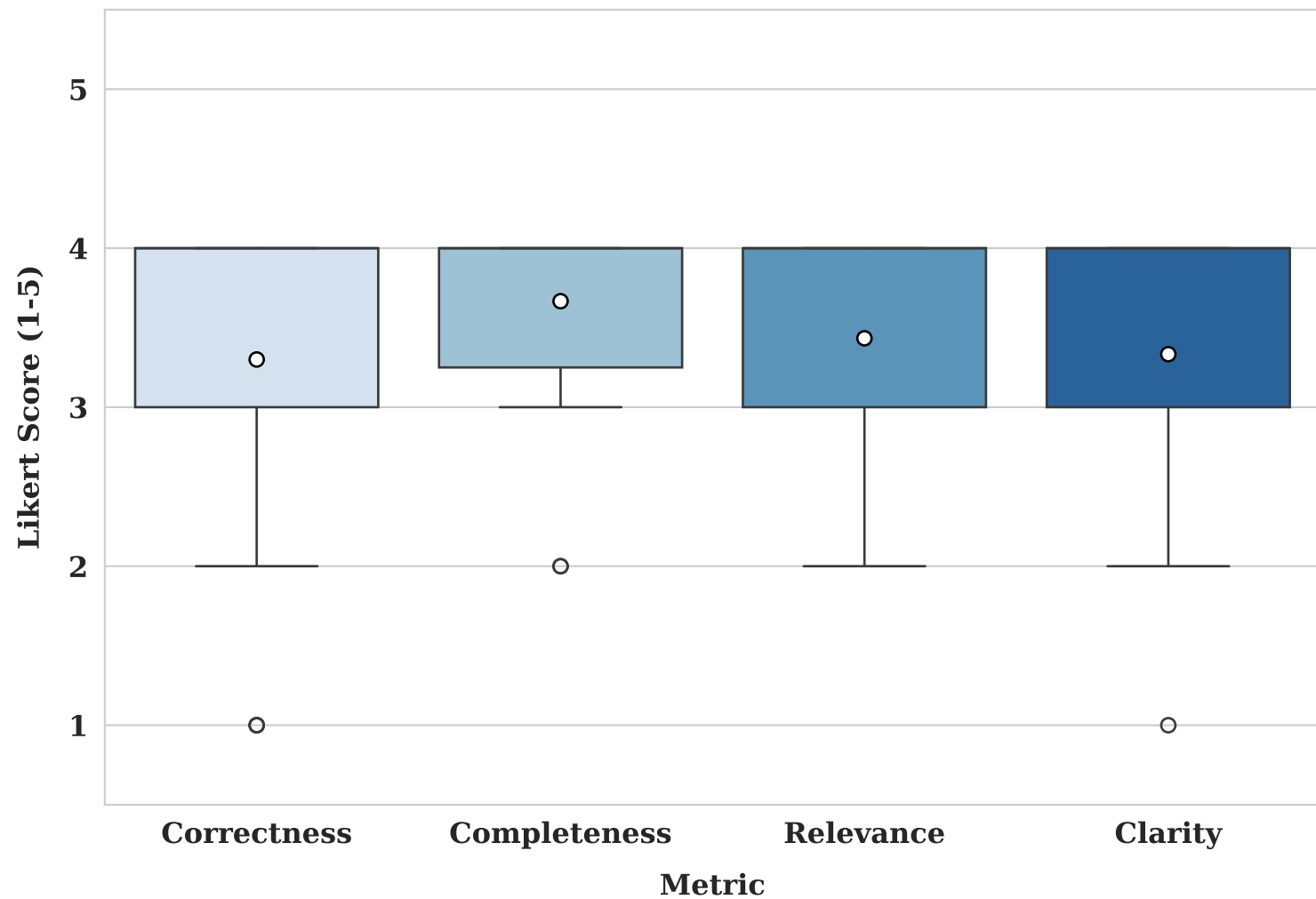
Overall Performance Distribution of RAG Chatbot
